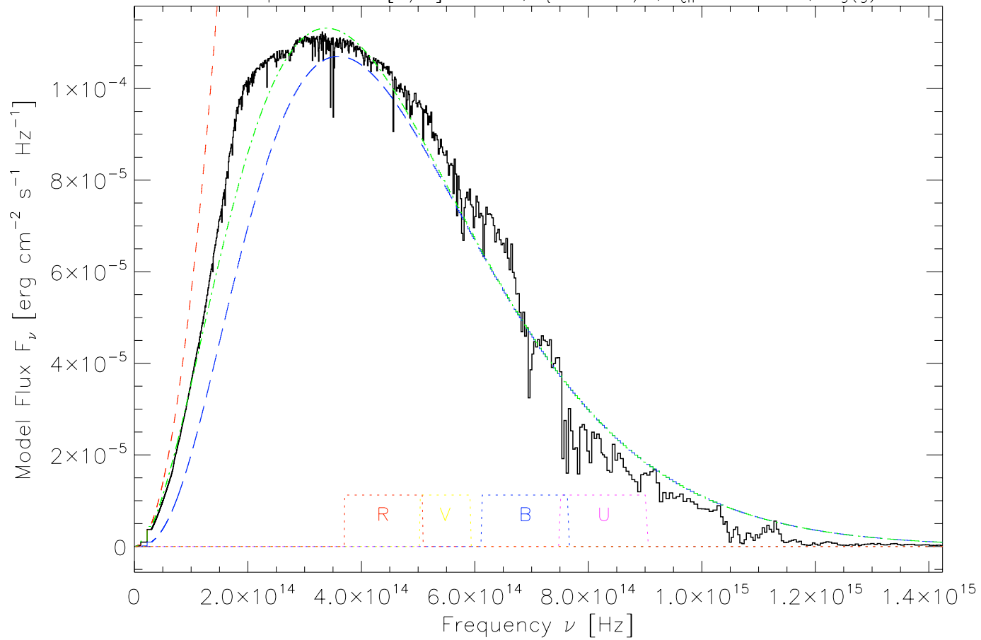
Kurucz model spectrum for [M/H] = +0.0 , v_t = 2 km/s, T_{\text{eff}} = 5750 K, \log(g) = +4.5
