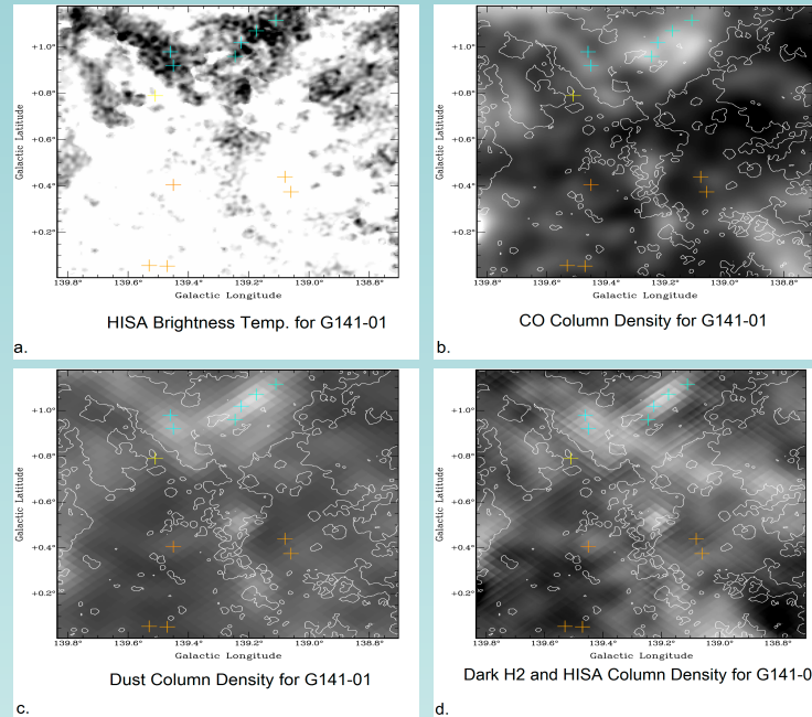
Maps of the cloud under investigation: (a) HISA channel map near the line peak showing the ON-OFF brightness difference (from Gibson et al. 2005); (b) ^{12}\text{CO} J=1-0 emission tracing "visible" H_2 content (Heyer et al. 1998), smoothed to the Planck resolution, integrated over velocity, and scaled by 2 X_{\text{CO}} = 3.6 \times 10^{20} \text{ cm}^{-2} (\text{K km/s})^{-1} for H-atom column density (Dame et al. 2001), with HISA contours overlaid; (c) Planck dust reddening ( Planck Consortium 2013), scaled to H-atom column density (Bohlin et al. 1978), with HISA contours; and (d) Planck dust column with HI emission and CO subtracted to show "dark" HI + H_2 column density, with HISA contours. Crosses in all panels mark target positions, for which results are tabulated. At the adopted distance of 2.3 kpc, 0.1 degree = 4 pc.
