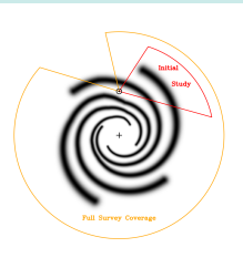
A schematic plan view map showing the CGPS Phase 1 area (red) and the larger coverage of the International Galactic Plane Survey area (yellow) that we plan to analyze in the future.
