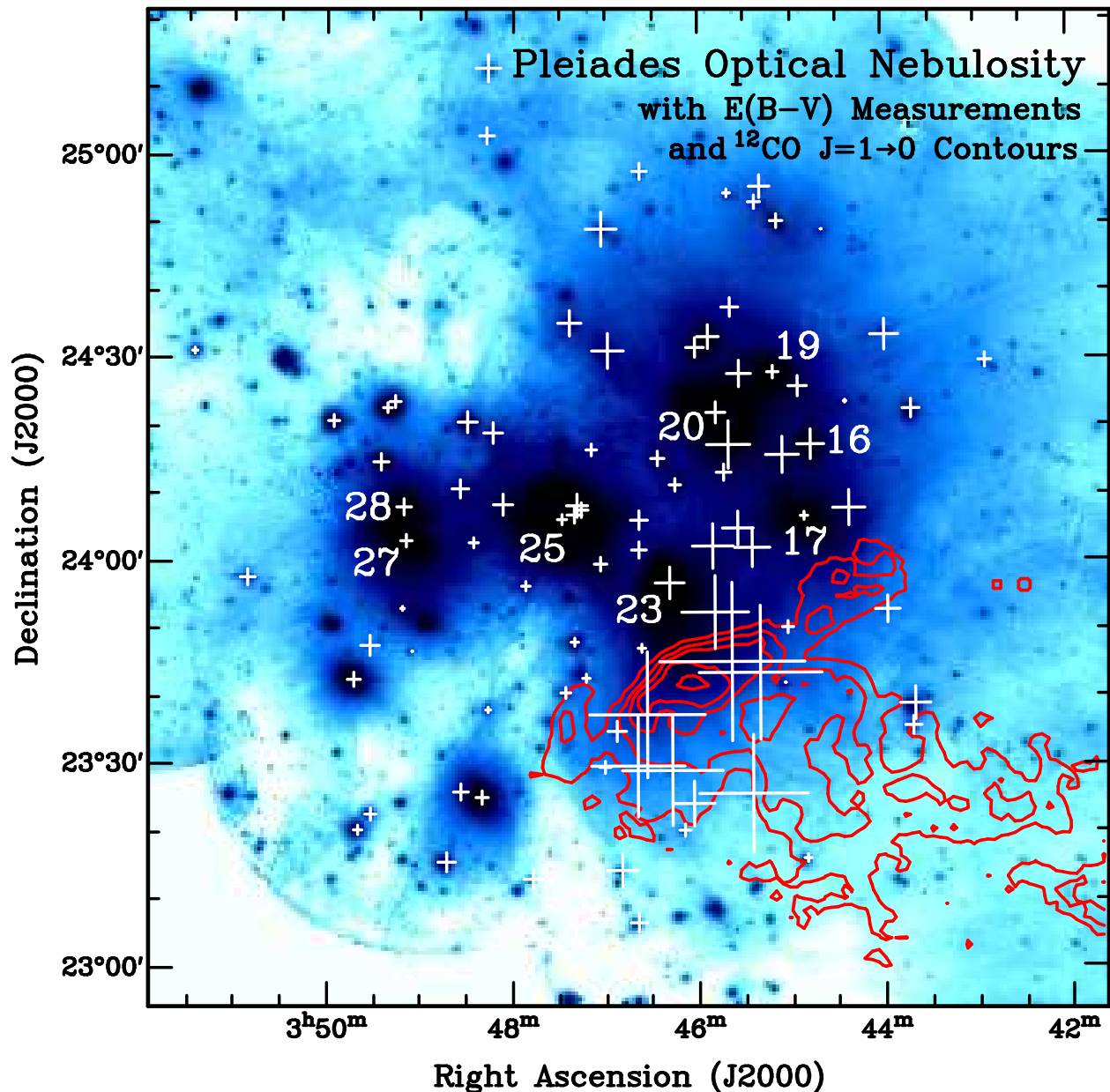
Fig. 1.— Interstellar reddening and molecular gas across the cluster core. Bright Flamsteed stars are numbered. The background is a log-scale negative image of 4400 Å nebulosity from Paper I, with intensities of 2.0 \times 10^{-19} - 2.0 \times 10^{-17} \text{ erg cm}^{-2} \text{ s}^{-1} \text{ \AA}^{-1} \text{ arcsec}^{-2} , or 26.3 – 21.3 B mag arcsec ^{-2} . Crosses show reddenings toward cluster members (Breger 1986), where E_{B-V} = \text{cross width in degrees} . The contours mark 5, 10, 15, 20, and 25 K km s ^{-1} profile integrals of ^{12}\text{CO } J = 1 - 0 emission from Bell Labs 7m telescope data provided by J. Bally & R. E. White (see Bally & White 1986). CH ^+ absorption is also detected toward a number of stars, with larger column densities measured for 16, 20, & 23 Tau than for 19, 25, & 27 Tau (White 1984).
