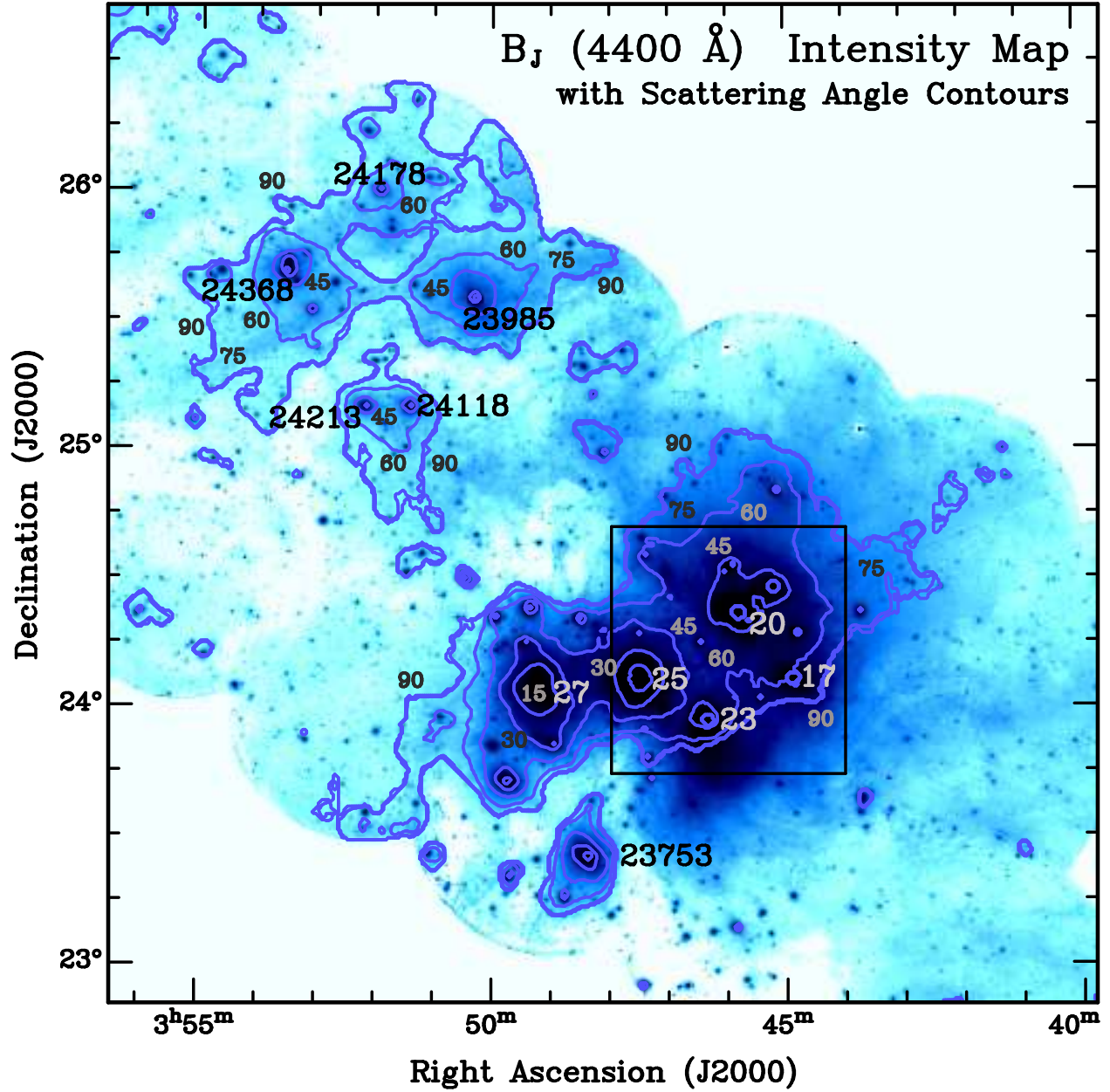
Fig. 8.— 4400 \text{ \AA} scattering angle contours for \theta = 15^{\circ} , 30^{\circ} , 45^{\circ} , 60^{\circ} , 75^{\circ} , and 90^{\circ} overlaid on Schmidt mosaic optical brightness from Paper I; the 75^{\circ} , and 90^{\circ} contours are often close together. The intensity scale is that of Fig. 1. The angles are calculated for a UV-modified Model A nebula (Table 3). Small numbers label selected contour values in degrees. Stars discussed in the text are labeled with larger Flamsteed and Henry Draper numbers. The box marks the area of Fig. 4.
