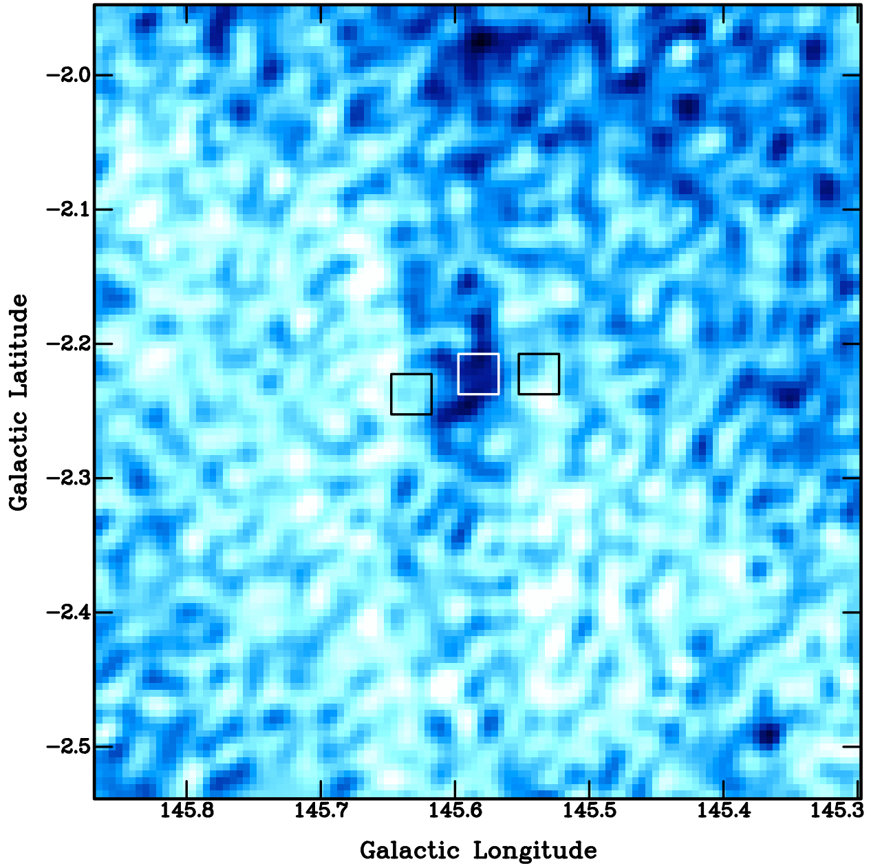
Fig. 3.— Example of a HISA feature at Local arm velocities, here 0 \text{ km s}^{-1} . Brightness temperatures displayed range from 55 K (black) to 90 K (white). No dust counterparts were found, and available CO data has insufficient angular resolution to show molecular gas on these scales. ON and OFF spectra were extracted from the 2' \times 2' white and black boxes, respectively.
